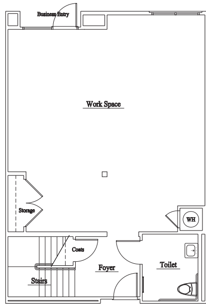
PLAN M
